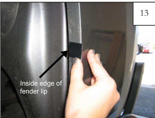
Center a supplied Tab (Item 8) over the six remaining marks made in Step 9, aligning edge of Tab with inside edge of fender lip (Tab may extend over outside of fender).
