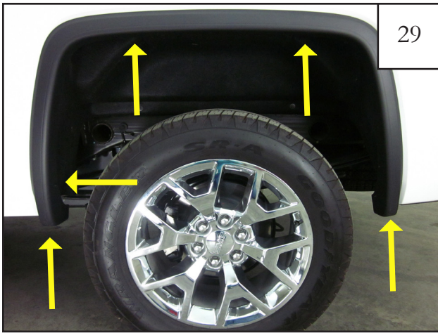
29 Remove fasteners from factory wheel arch molding using a T-15 Torx Bit for upper and lower wheel well fasteners and a 10mm deep socket and wrench for the lower 2 locations.
